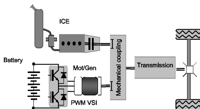
Figure 3. Parallel HEV
