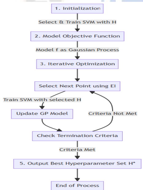
FIG1:Flow diagram for Bayesian Optimization with SVM
