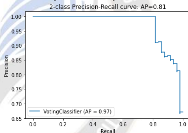
Fig.5: Precision-Recall curve of Voting Classifier
