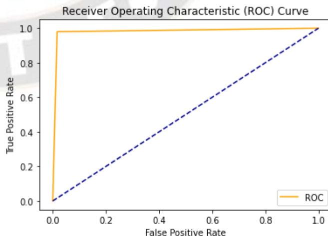
Fig. 6: ROC of Bagging Classifier
