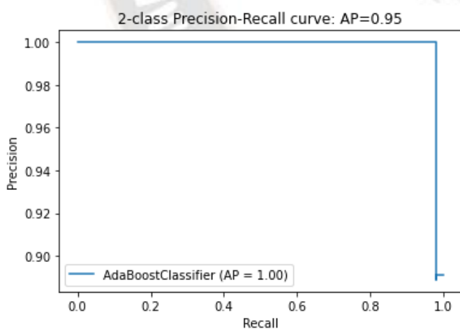
Fig. 9: Precision-Recall Curve of AdaBoost Classifier
