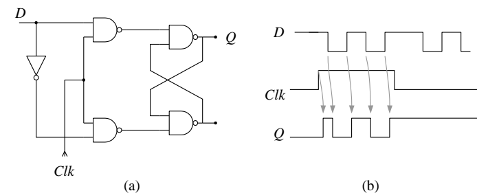
Figure 2: (a) Clocked D-Latch (b) timing diagram of clocked D-Latch So as to make it perfect with the synchronous structure we will confine when Q can be influenced by presenting the clock signal which entryways S and R inputs. On the off chance that the information input D is associated with S, and the property of S-R lock, which makes S and R totally unrelated is connected, the subsequent D hook is appeared in Fig.2 (a). The related planning graph of a D-Hook is appeared in Fig. 2 (b). The hook is straightforward amid the timeframe in which clock is dynamic, – for example expecting rationale 1 esteem.
