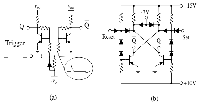
Figure.6: (a) Early version of a Flip-Flop (b) PDP-8 direct Set-Reset sequential element
