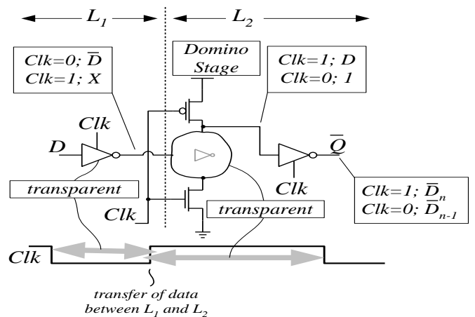
Figure 4: TSPC Latch operation
