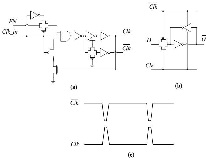
Figure 5: Pulse Latch: (a) local clock generator, (b) single latch (c) clock signals
