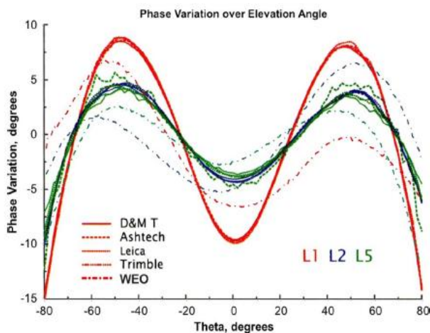
Figure 3 Comparison of measured phase variation of five high-performance GNSS antennas.
