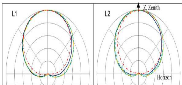
Figure 4 Radiation pattern of conventional Antenna
