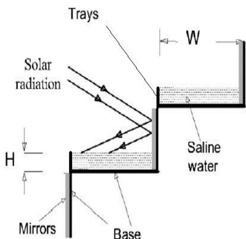
Fig.1.2 Trays and mirrors on the steps of the modified stepped still. [4]
