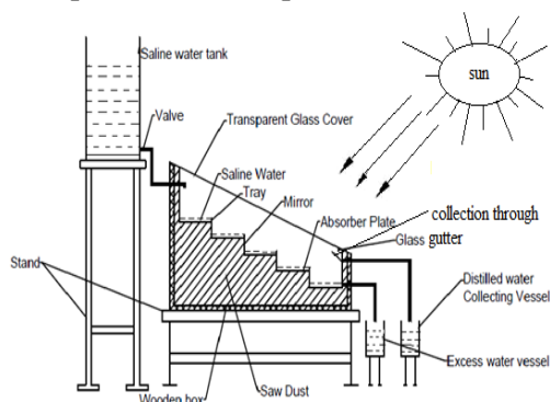
Fig 1.3 SCHEMATIC DIAGRAM OF STEPPED BASIN TYPE SOLAR STILL
