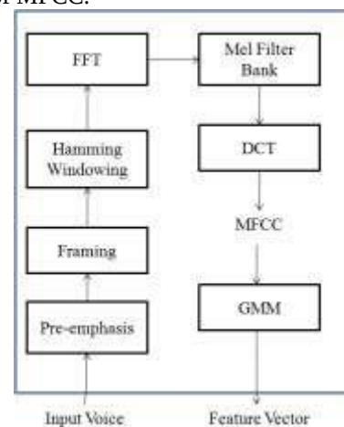
Figure 2. Computational Steps for Speaker Recognition
