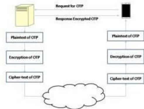
Figure 3. Implementation of OTP System
