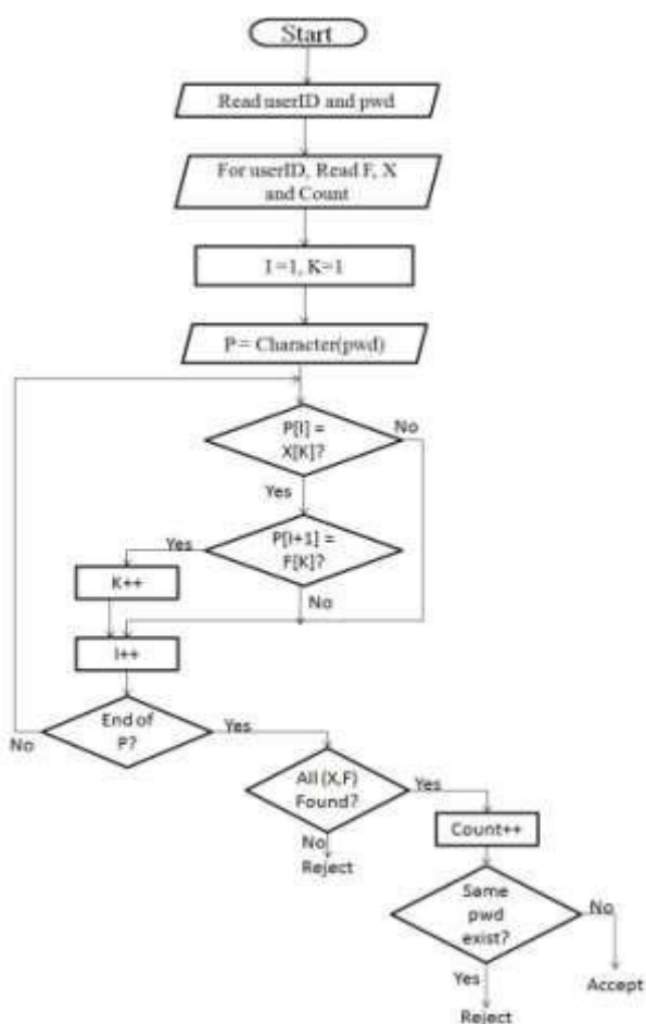
Figure 1. Extraction of Actual Password from Password String
