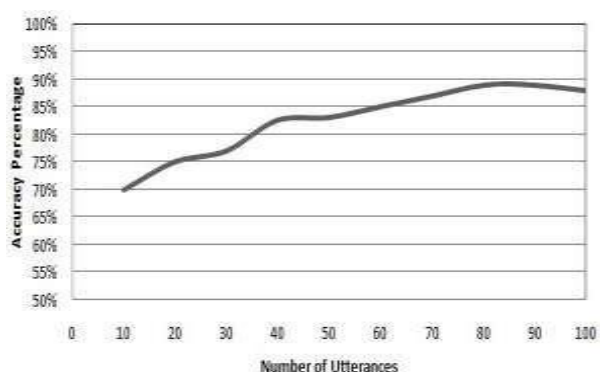
Figure 4. Performance of GMM
