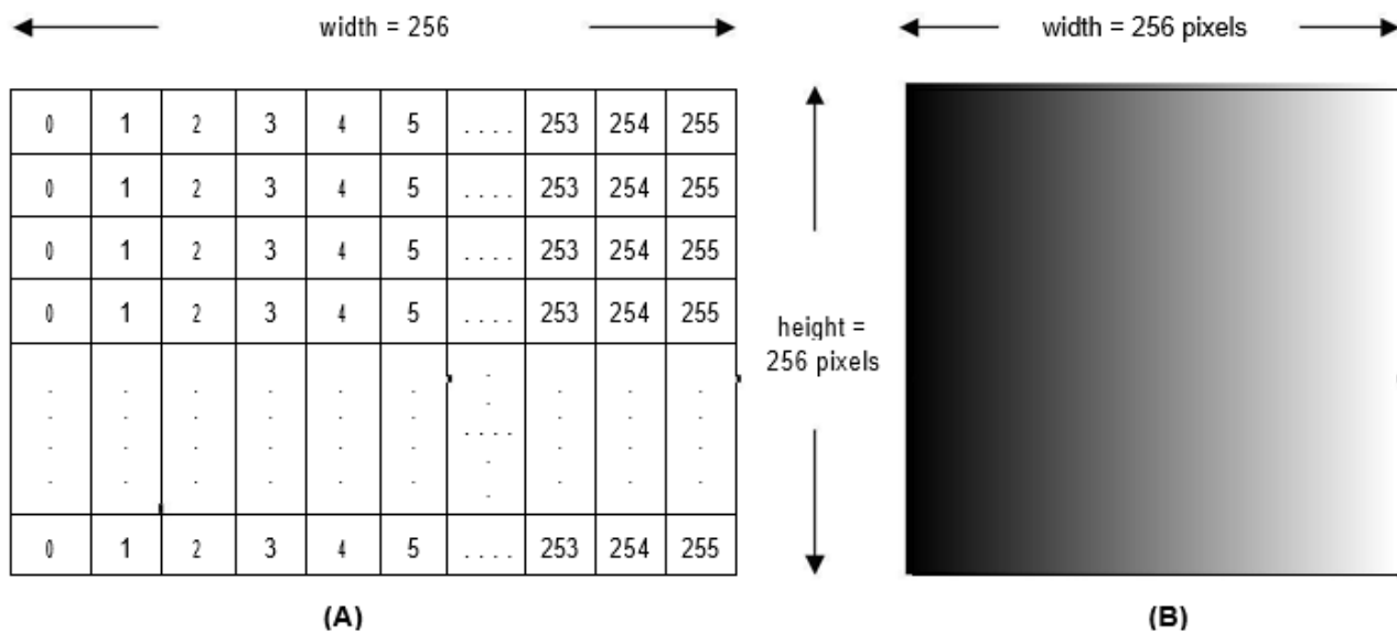
Figure: Values in the grid represent the grayscale intensities of the image on the right. (A) Intensity values are shown in a grid of the same dimension as image (B) Image as seen on a monitor
