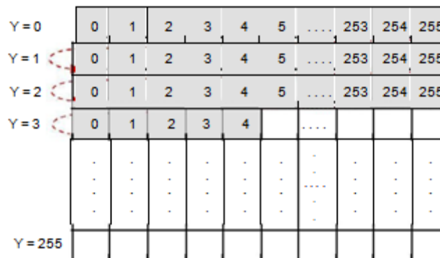
Figure: Array traversal in a 'for' loop. Note that rows are being accessed one after the other. This is known as 'Row Major Traversal'. The graphic suggests that in the current iteration, x = 4 and y = 3 both starting from 0.
