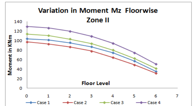
Figure-27 Moment Mz for Zone II (Corner Column)
