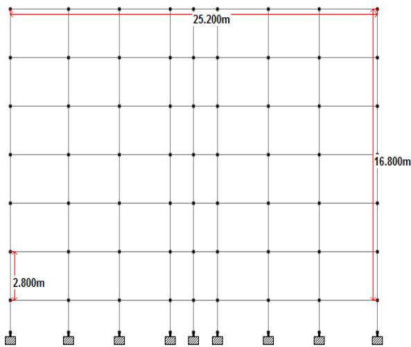
Figure-2 Elevation of Structure
