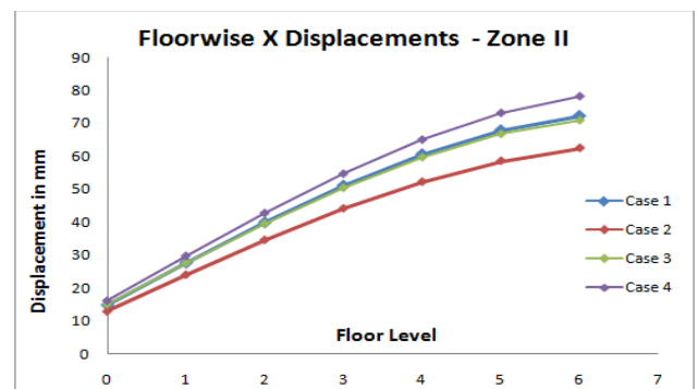
Figure-9 X displacement for Zone II (Intermediate Column)
