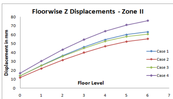
Figure-13 Z displacement for Zone II (Intermediate Column)
