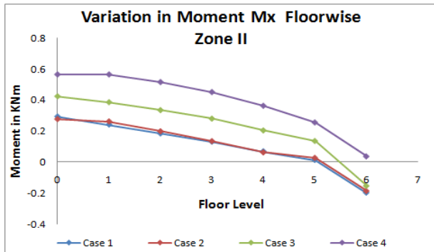
Figure-23 Moment Mx for Zone II (Corner Column)
