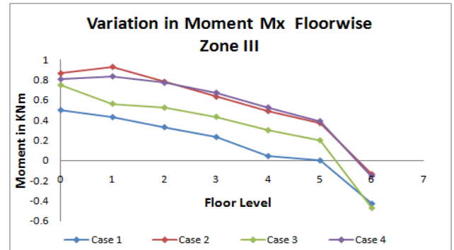
Figure-26 Moment Mx for Zone III (Intermediate Column)
