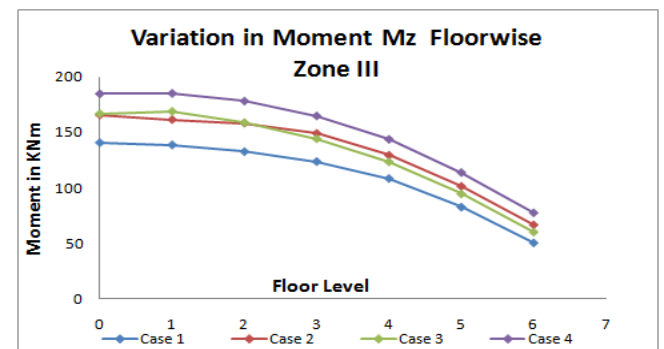
Figure-28 Moment Mz for Zone III (Corner Column)
