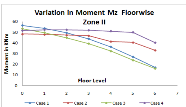
Figure-31 Moment Mz for Zone II (Corner Beam)
