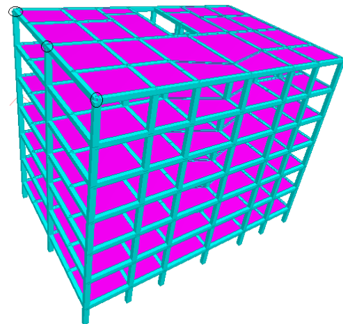
Figure-4 External Floating Column (case 2)
