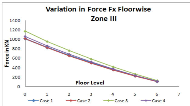
Figure-18 Axial Force F_x for Zone III (Intermediate Column)
