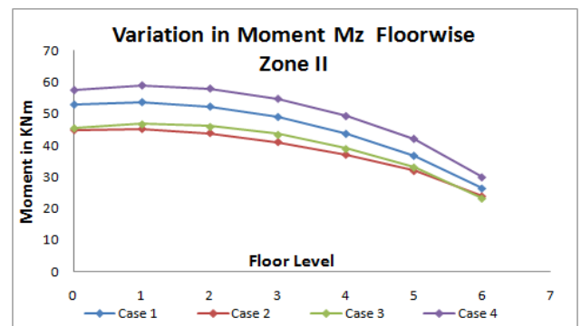
Figure-33 Moment Mz for Zone II (Intermediate Beam)
