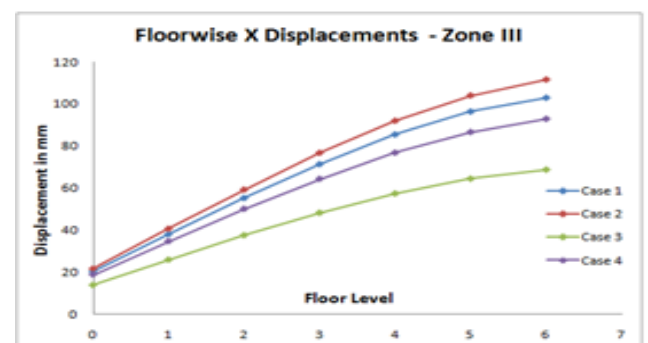
Figure-10 X displacement for Zone III (Intermediate Column)
