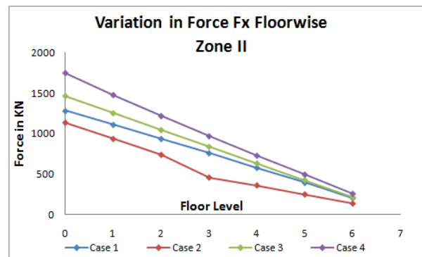
Figure-15 Axial Force Fx for Zone II (Corner Column)
