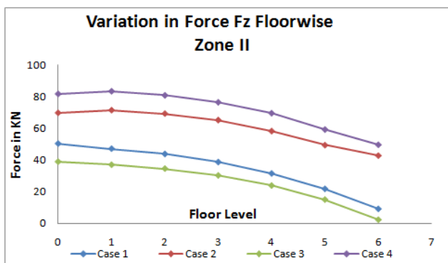
Figure-19 Shear Force F_z for Zone II (Corner Column)
