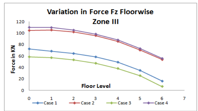
Figure-20 Shear Force F_z for Zone III (Corner Column)
