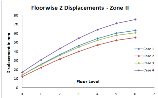
Figure-11 Z displacement for Zone II (Corner column)
