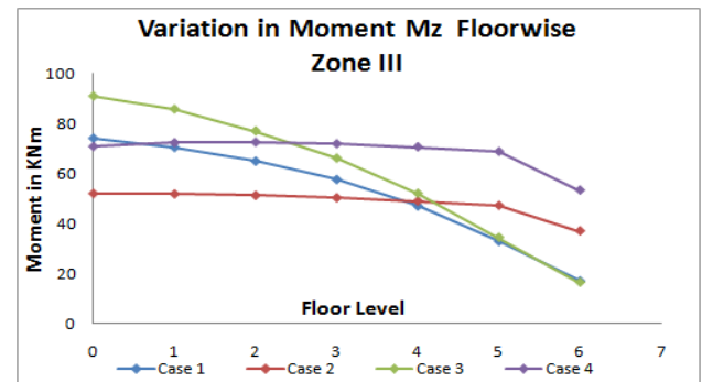
Figure-32 Moment Mz for Zone III (Corner Beam)
