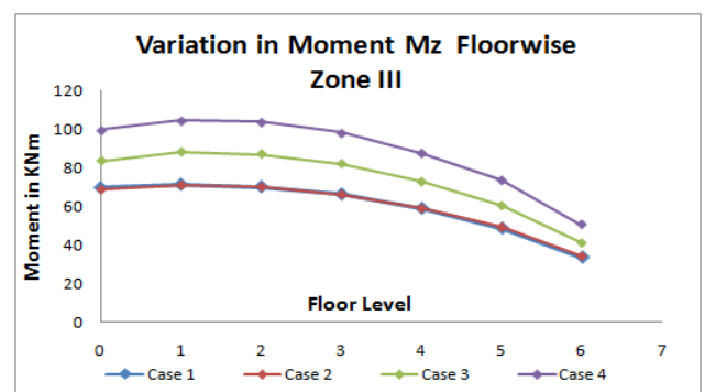
Figure-34 Moment Mz for Zone III (Intermediate Beam)
