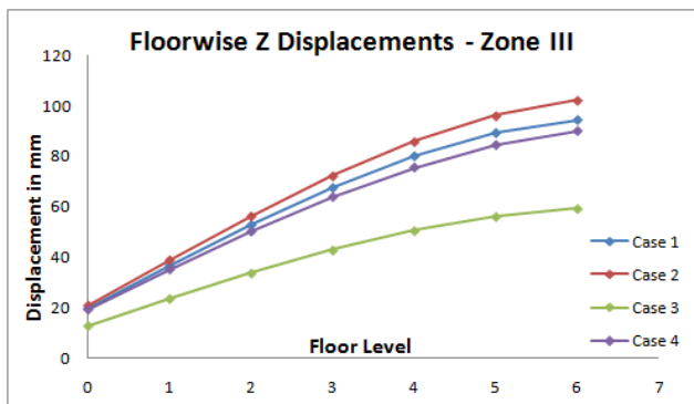
Figure-12 Z displacement for Zone III (Corner column)
