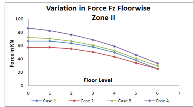
Figure-21 Shear Force F_z for Zone II (Intermediate Column)
