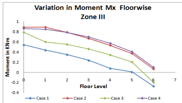
Figure-24 Moment Mx for Zone III (Corner Column)
