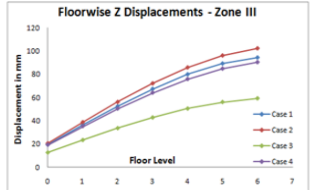
Figure-14 Z displacement for Zone III (Intermediate Column)
