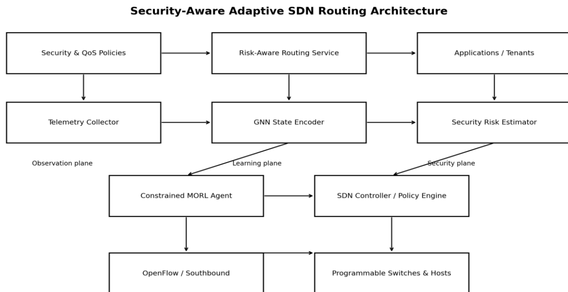
Fig. 1. Overall architecture of the proposed Security-Aware Risk-Guided Multi-Objective Reinforcement Learning (SARG-MORL) framework.
