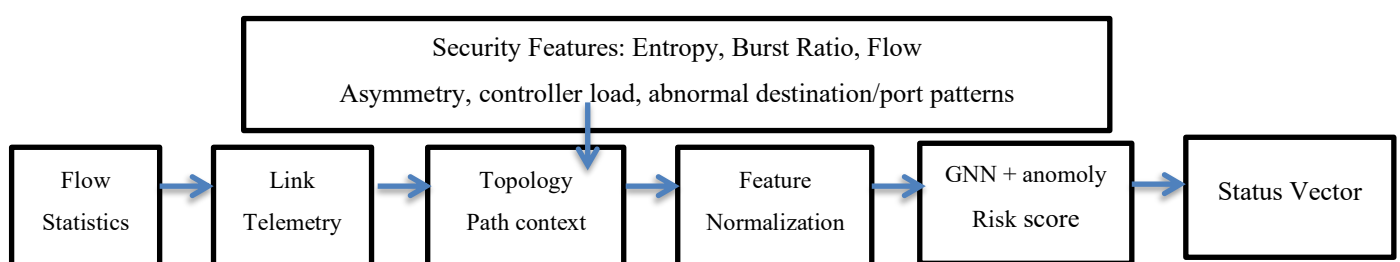
Fig. 2. Telemetry collection and security-aware state construction pipeline.
