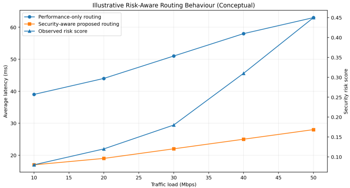
Fig. 5. Conceptual illustration of risk-aware routing behavior. This figure is methodological, not an experimental result; replace with measured data before submission.
