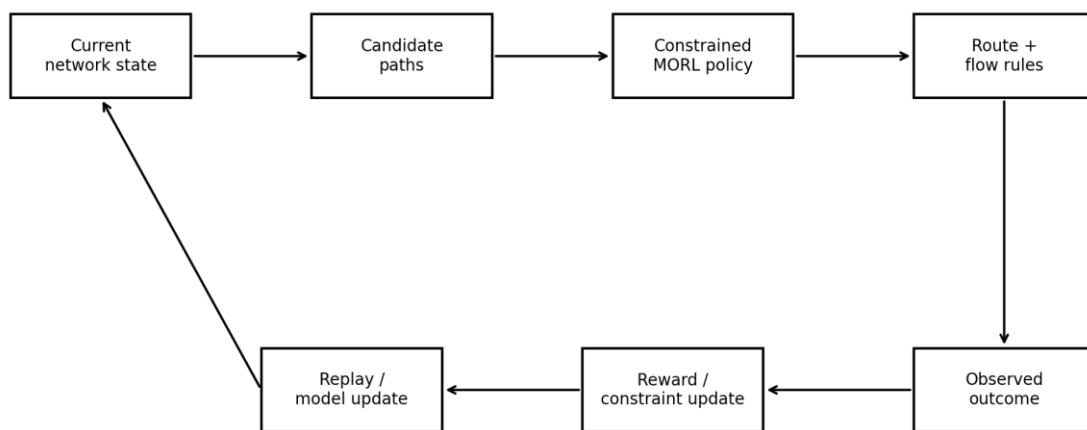
Security-Constrained Multi-Objective Routing Decision Loop
