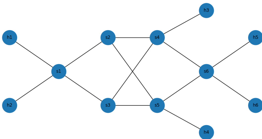
Fig. 4. Representative Mininet experimental topology used for reproducible SDN evaluation.
