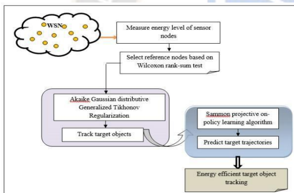
Figure 1 Architecture Diagram of Proposed GG-DSRP method
