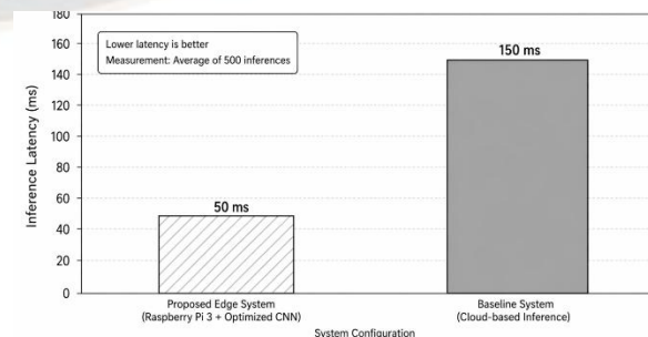
Figure 4: Latency Comparison
