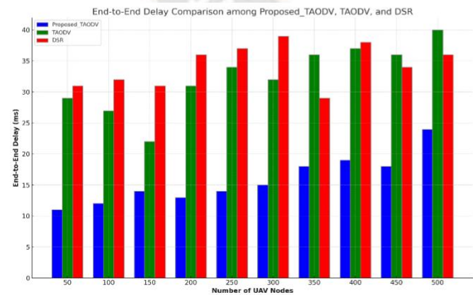
Figure 2. End-to-end delay, measured in milliseconds (ms) The table 3 and figure 2 provides an analysis of end-to-end delay, measured in milliseconds (ms), for three different protocols—Proposed_TAODV, TAODV, and DSR—as the number of UAV nodes increases from 50 to 500. The data
