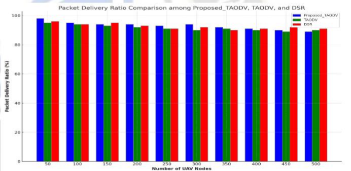
Figure 3. Packet delivery ratio (PDR), expressed as a percentage The table 4 and figure 3 shows the packet delivery ratio (PDR), expressed as a percentage, for Proposed_TAODV, TAODV, and DSR protocols across varying numbers of UAV nodes, ranging from 50 to 500. Proposed_TAODV starts with a PDR of 98% at 50 UAV nodes and gradually decreases to 89% at 500 nodes, showing a slight but consistent decline as the number of nodes increases. TAODV begins with a PDR of 95% and experiences a slight fluctuation, ultimately reaching 90% at 500 nodes, indicating a modest decrease in delivery efficiency with network expansion. DSR, meanwhile, starts at 96%, peaks at 95% for 150 nodes, and then slightly decreases to 91% by 500 nodes, demonstrating relatively stable performance with a mild decline over a broad range of node counts. This data illustrates the overall robustness of Proposed_TAODV in maintaining higher delivery ratios compared to TAODV and DSR, particularly in denser UAV networks.
