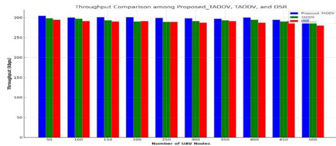
Figure 1. Comparison of throughput performance (kbps) The table 2 and figure 1 presents a comparison of throughput performance (kbps) across different numbers of Unmanned Aerial Vehicle (UAV) nodes for three protocols: Proposed_TAODV, TAODV, and DSR. As the number of UAV nodes increases from 50 to 500, the throughput for Proposed_TAODV slightly decreases from 304 to 297, demonstrating relatively stable performance. TAODV's throughput also shows a slight decrease from 298 to 291, with minor fluctuations. DSR exhibits a more variable performance, starting at 294 and ending at 280, with both increases and decreases throughout. Overall, Proposed_TAODV consistently outperforms TAODV and DSR across all node counts, indicating its superior efficiency in handling increasing numbers of UAV nodes.
