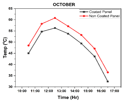
Figure 8. Temperature comparison of two panels in the months of (a) August (b) September (c) October
