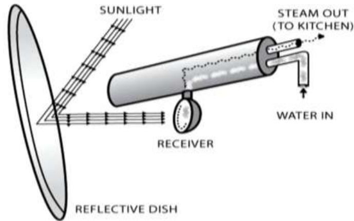
Fig. Working of parabolic dish solar collector for steam generation
