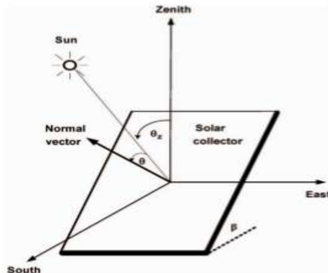
Fig.2 Geometry of solar collector
